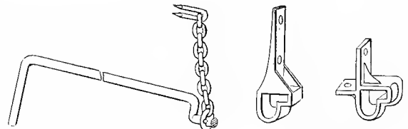
Figs. 2231-2232. Bracket for Face of End-sill, Corner of Sill.
